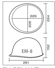
EM-8型寸法図
