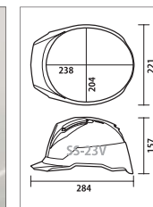
SS-23V型寸法図
